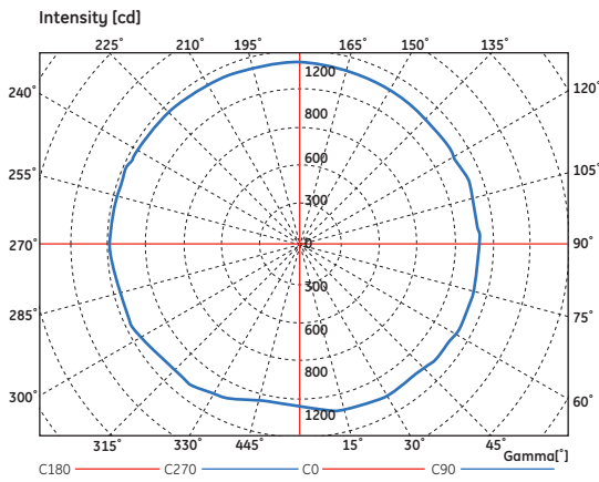
CMH G12 150W
