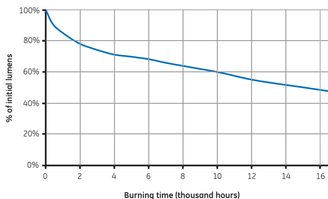
Lumen maintenance CMH G12 35W 3000K
