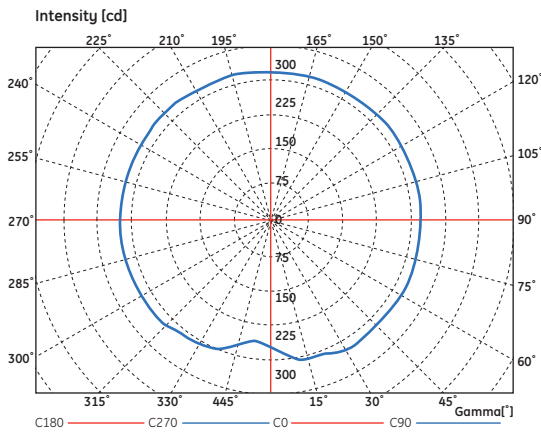
CMH G12 70W
