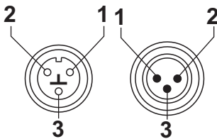
DMX signal connector
